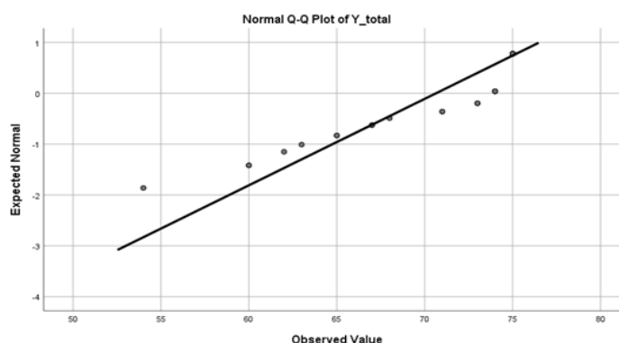
Gambar 2. Normal Q-Q Plot of Y_total
