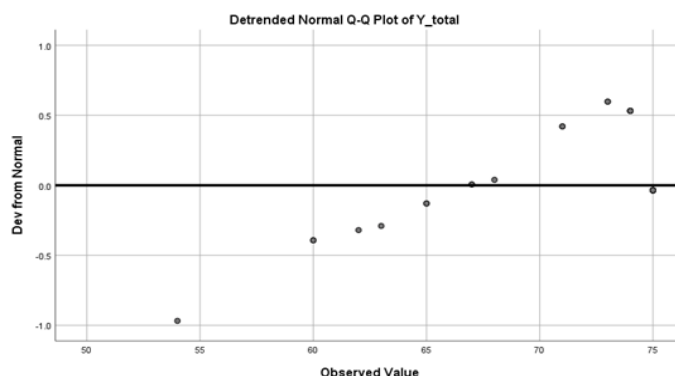
Gambar 3. Detrended Normal Q-Q Plot of Y_total
